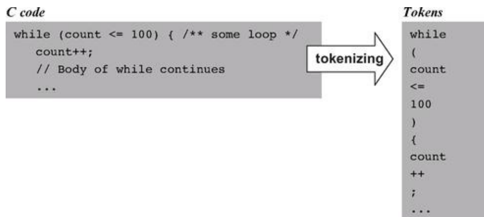
Figure 10.2 Lexical analysis.
