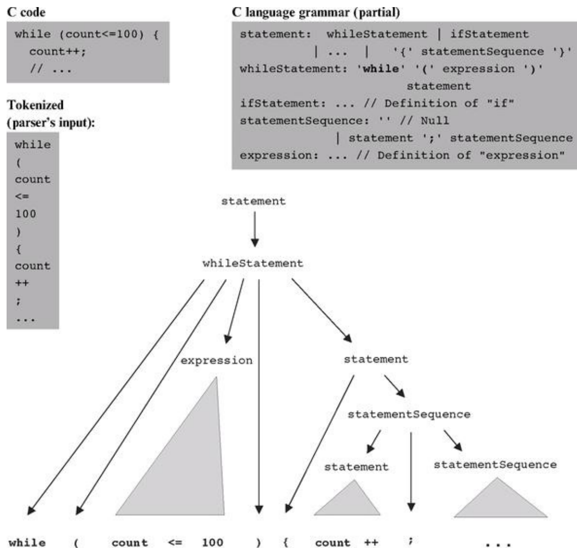
Figure 10.4 Parse tree of a program segment according to a grammar segment.
