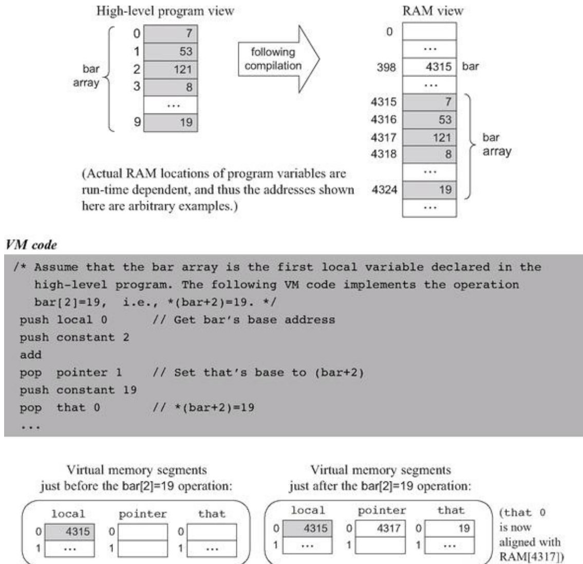
Figure 7.10 VM-based array manipulation using the pointer and that segments.
