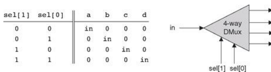
Figure 1.11 4-way demultiplexor.
