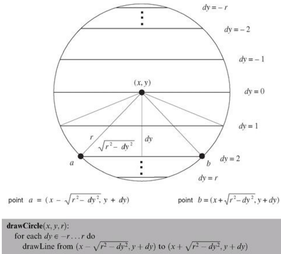
Figure 12.9 Circle drawing.
