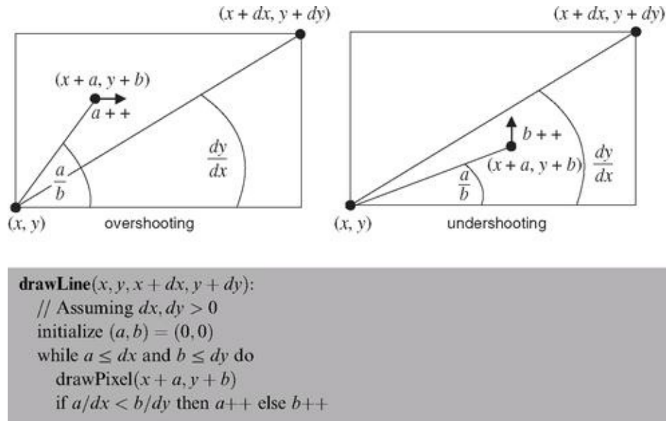
Figure 12.8a Line drawing.
