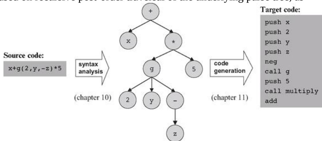
Figure 11.4 Code generation.
